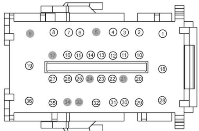
Connector C2280C
