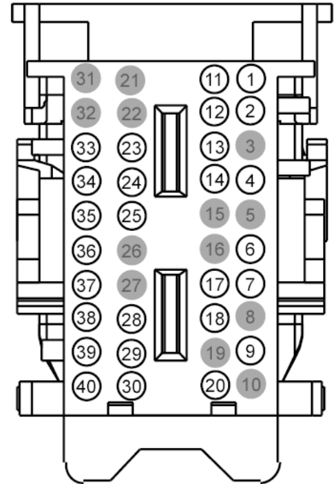
Connector C2280F
