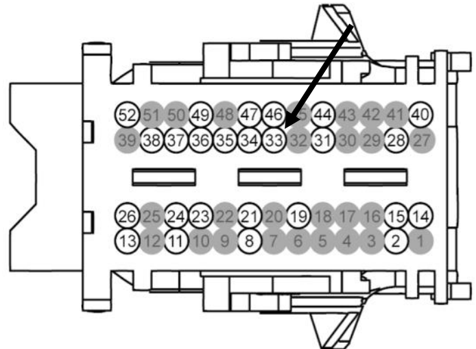
Connector C2280E
