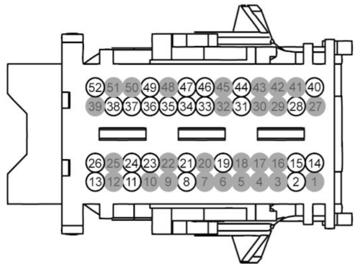
Connector C2280E
