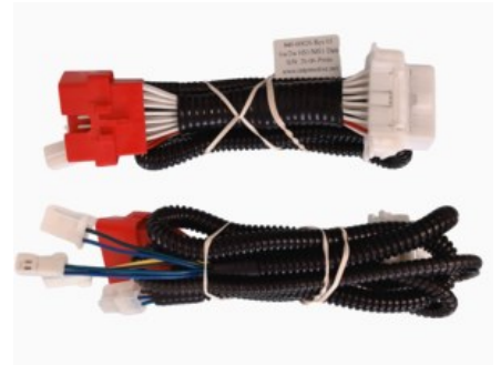
Harness 840-00124
