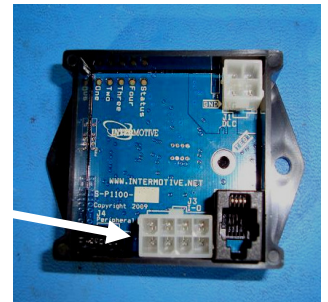
8 Pin lift connector
