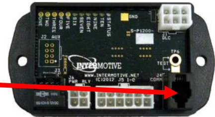
J4 COMM Port
