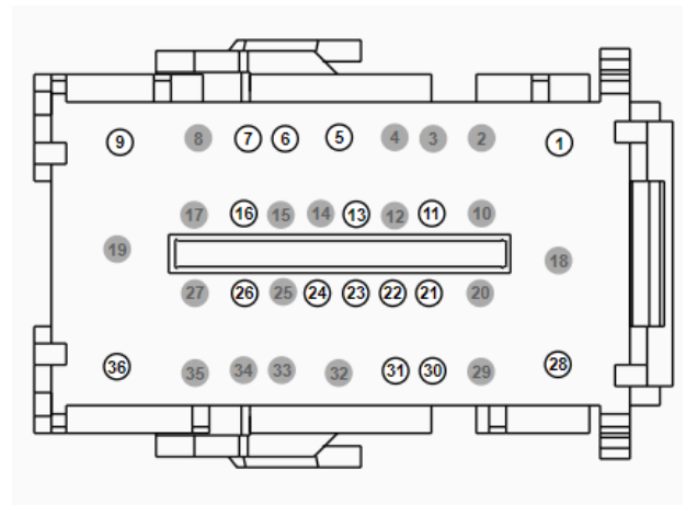
Connector C2280B
