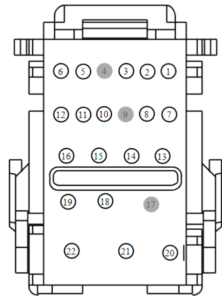
Connector C2280C
