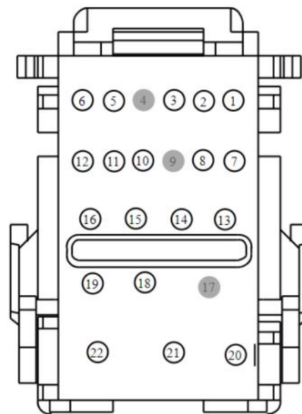
Connector C2280C
