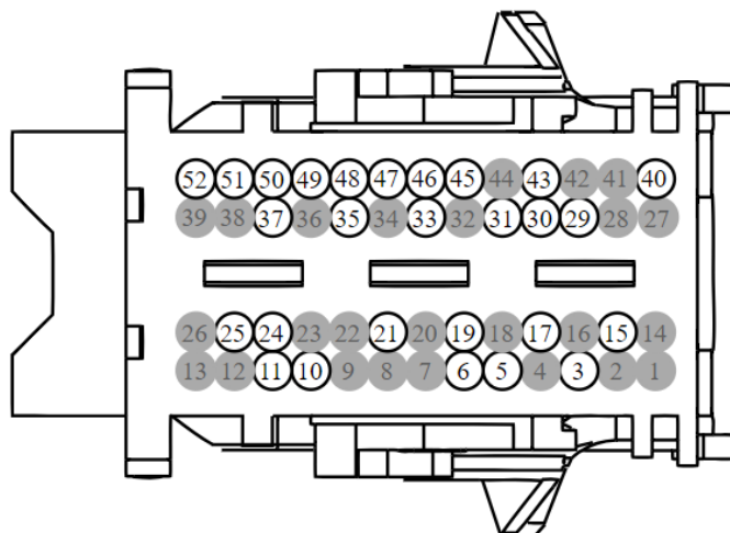
Connector C2280D
