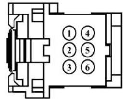
C2195 Front of Connector
