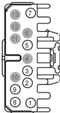
2009-19 E-Series C250 Front of Connector
