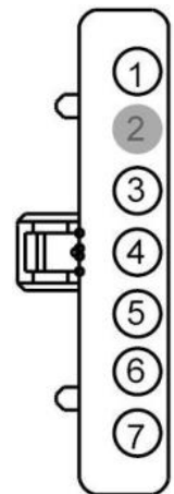
2011-'22 F-Series, 2020-'21 Transit, 2021-'24 E-Series C250 Front of Connector
