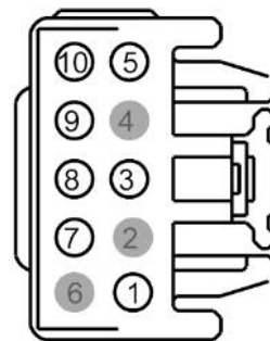
2008-10 F-Series C250 Front of Connector
