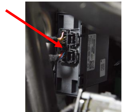
Durango gateway module with 8 & 12 pin connectors.
