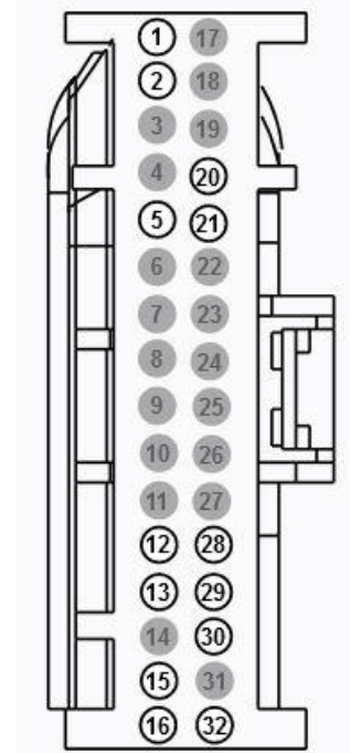
Connector C2280D
