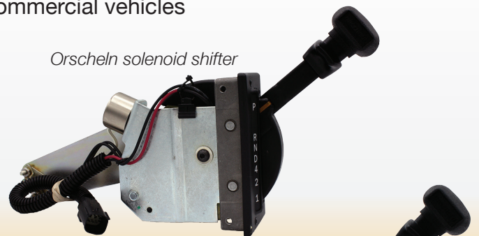
Orscheln shifter with custom solenoid for InterMotive application
