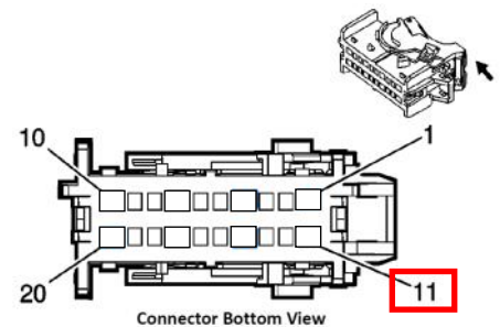
Connector Bottom View
