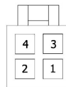
Back of Connector
