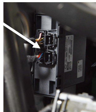
Charger gateway module with 8 & 12 pin connectors.
