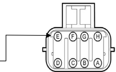
Front of the C314 Transmission Body Builder Connector
