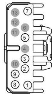
Connector C250
